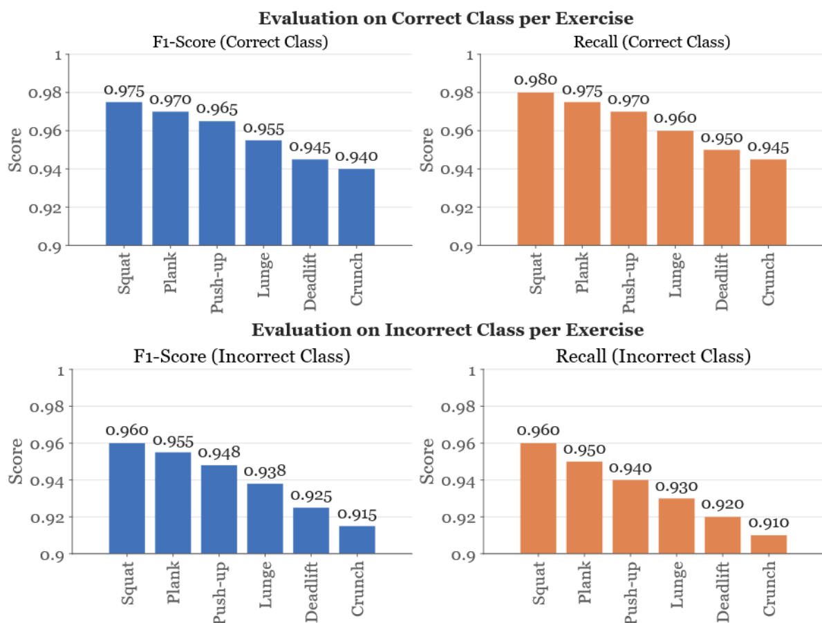
Figure 4. F1-score and recall of the proposed model for correct (top) and incorrect (bottom) executions across movement complexity (0–1 scale).
